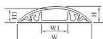
弧形配线槽 Round type wiring duct
